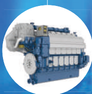
3 X DUAL-FUEL (DIESEL + LNG) 6L34DF WARTSILA 2850 kW e
